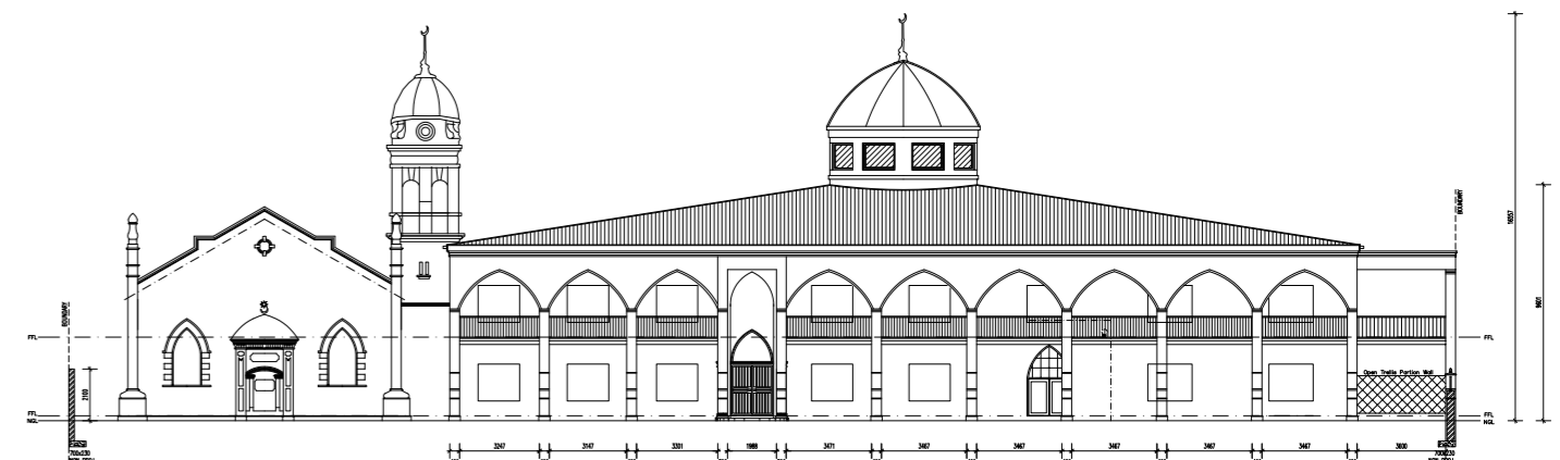
NORTH ELEVATION
